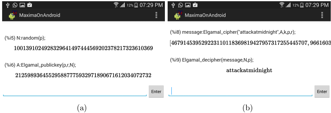
Figure 2: Elgamal cryptosystem
