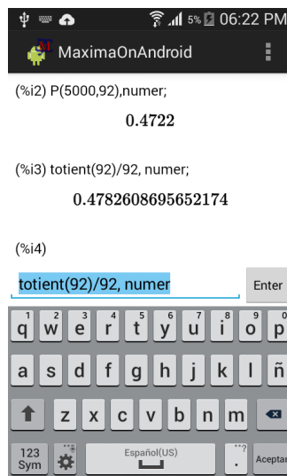
Figure 1: The totient function
