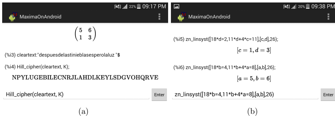
Figure 3: Hill cryptosystem
